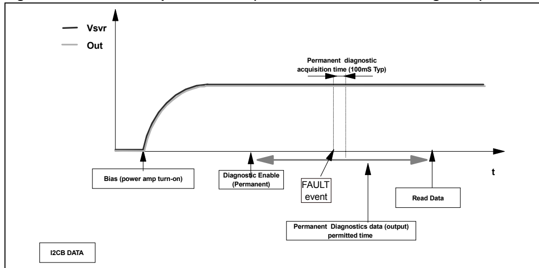
Figure 18. SVR and Output pin behaviour (CASE 2: with turn-on diagnostic)
