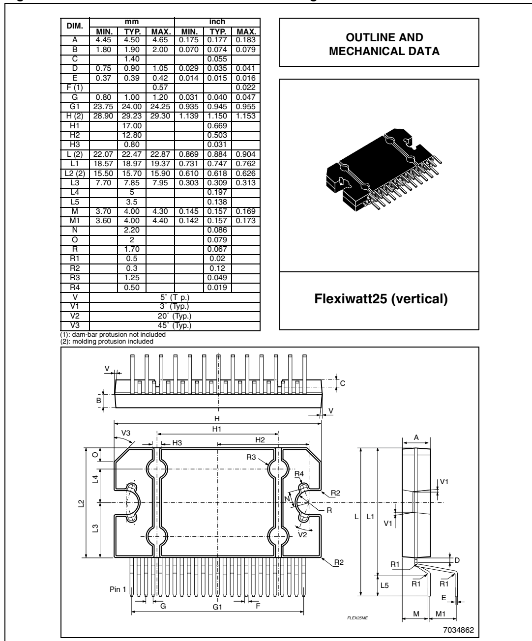
Figure 28. Flexiwatt25 Mechanical Data & Package Dimensions
